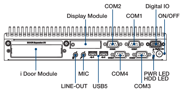
Rear Panel External I/O Mechanical Layout/Drawing
